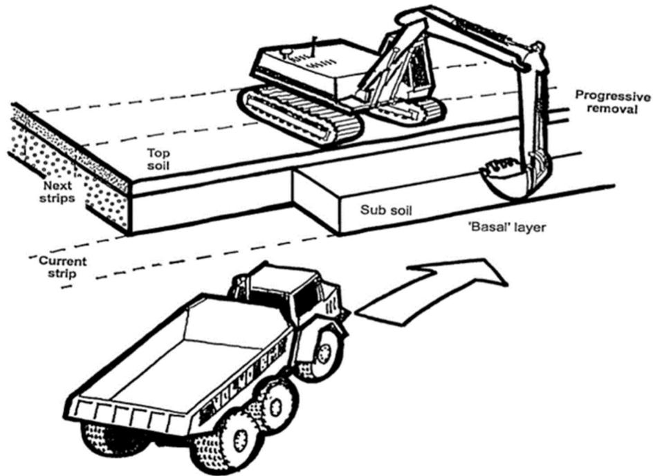
Plate 2: Stripping with excavators and dump trucks: removal of subsoil from a strip. Reproduced from Sheet A of the Good Practice Guide for Handling Soil (Institute of Quarrying, 2021) MAFF, 2000 (Ref: 1-2)
