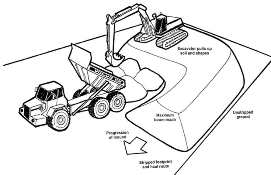
Plate 3: Soil storage mound construction with excavators and dump trucks. Reproduced from MAFF, 2000 (Ref: 1-2) the Good Practice Guide for Handling Soil (Institute of Quarrying, 2021)
