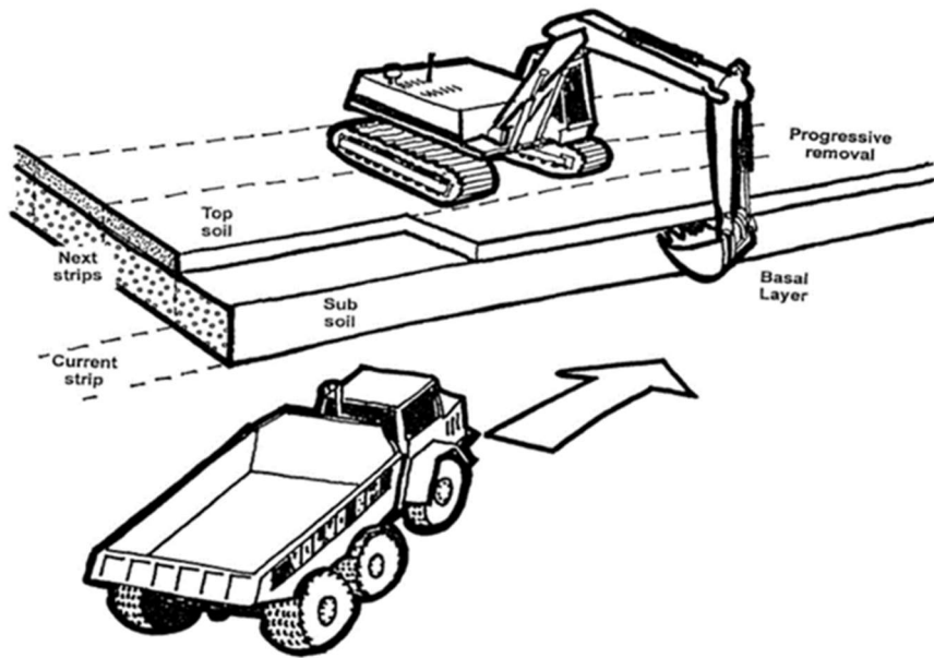
Plate 1: Stripping with excavators and dump trucks: removal of topsoil from a strip. Reproduced from MAFF, 2000 (Ref: 1-2) Sheet A of the Good Practice Guide for Handling Soil (Institute of Quarrying, 2021)
